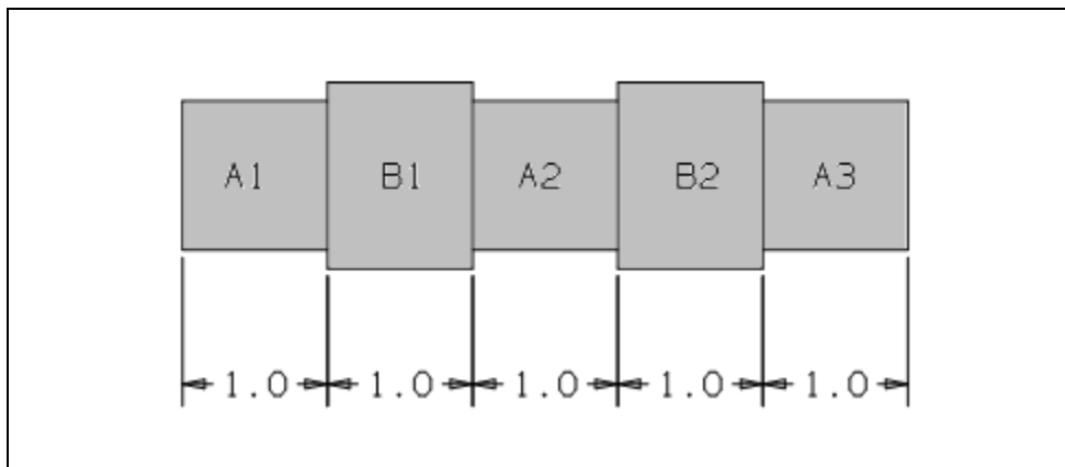
Figure 1, Unassigned Datum
