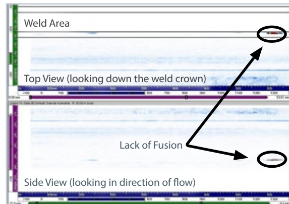
Flaw 4: Lack of Fusion Length: 0.327"
